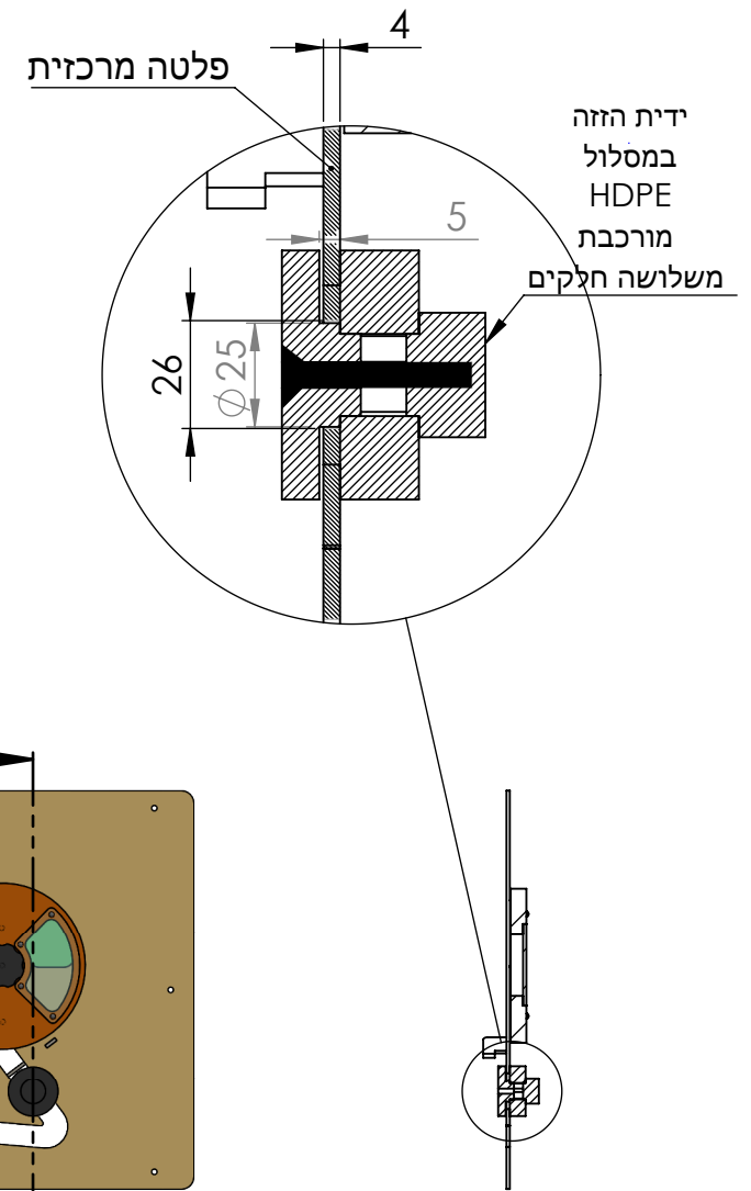
SECTION L-L SCALE 1 : 10
